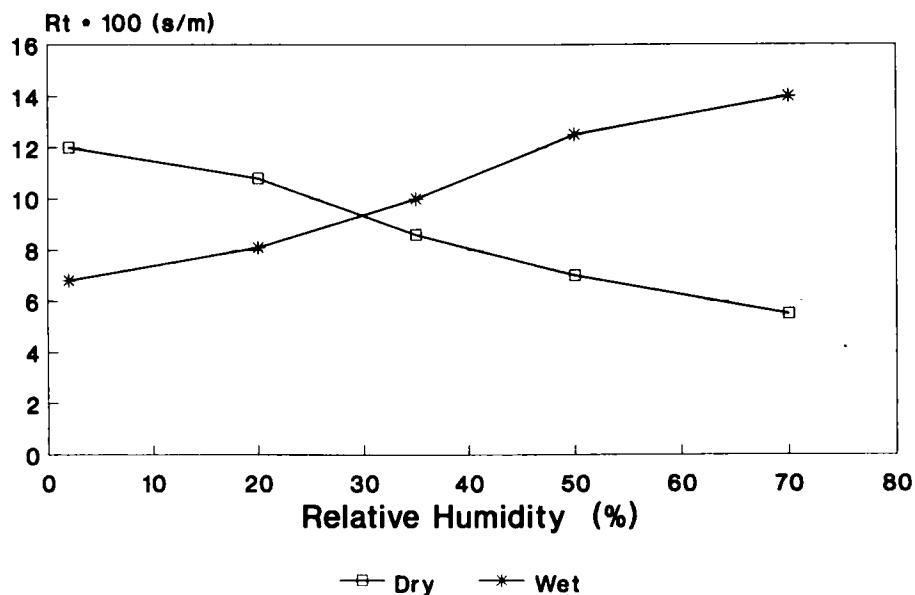
Figure 4 Influence of humidity on R 1 W-badges prepared by using the TEA solution.
