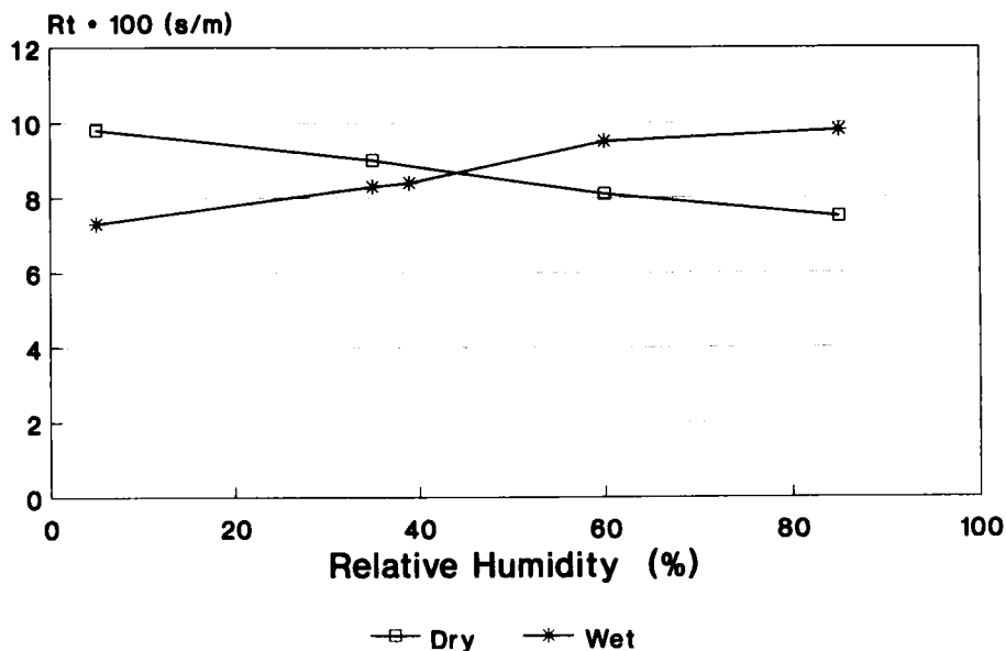
Figure 3 Influence of humidity on R 1 W-badges prepared by using the carbonate solution.
